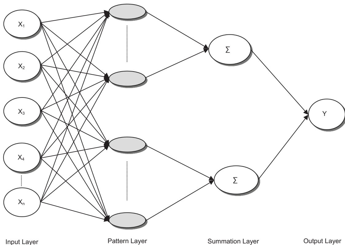
Fig. 2. Architecture of Generalized Regression Neural Network (GRNN).
