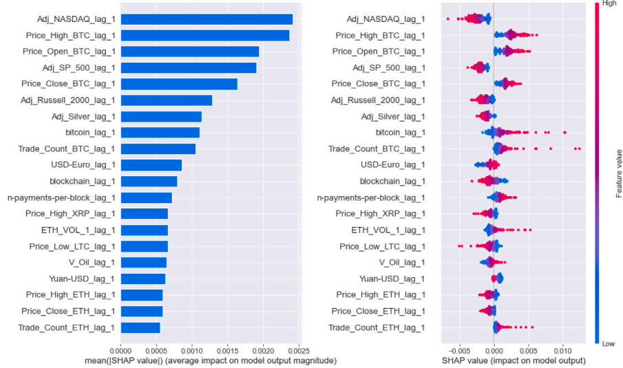
Fig. 6. SHAP summary of VOL_1 for Bitcoin using universal LSTM.
