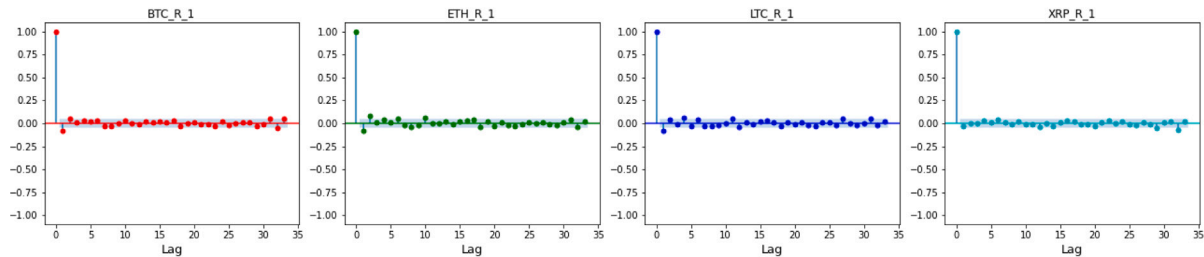
(a) ACF of Daily Return
