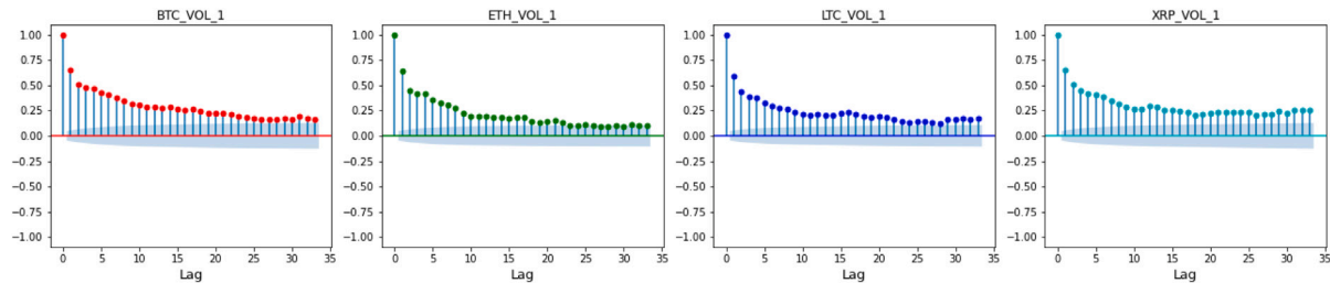
(a) ACF of Daily Volatility
