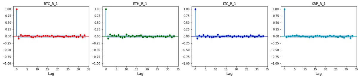
(b) PACF of Daily Return
