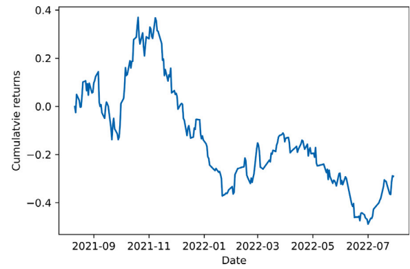
Fig. 8. Cumulative daily returns of Bitcoin.
