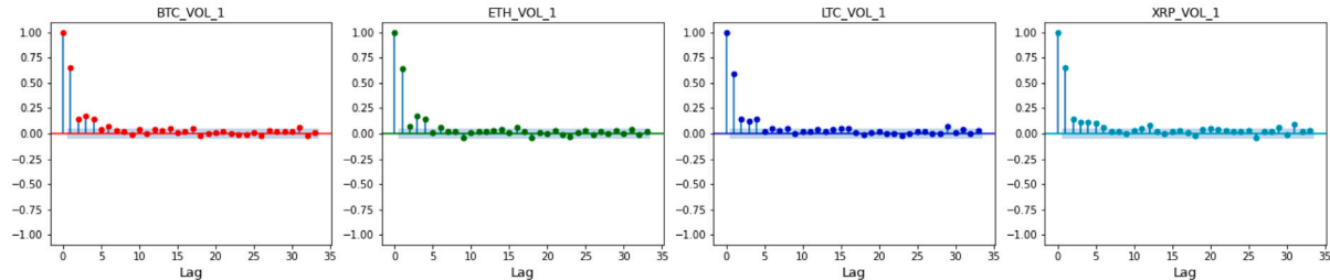
(b) PACF of Daily Volatility
